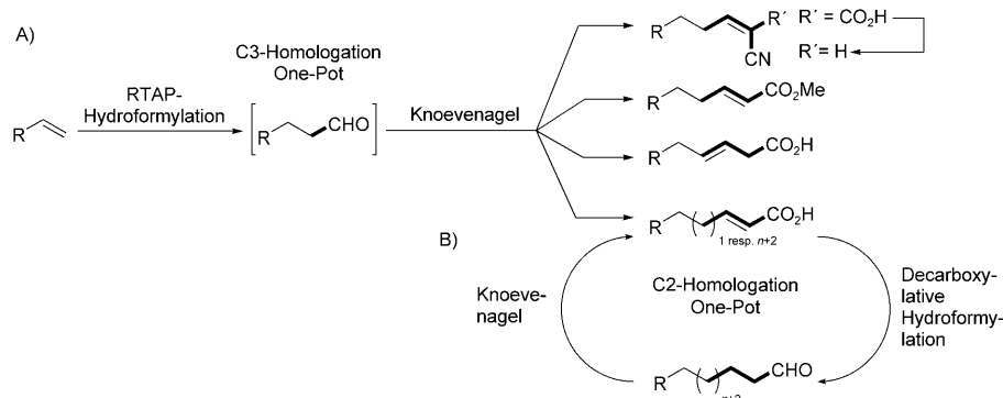
Scheme 3. Combined transition-metal- and organocatalysis—a new approach to carbonyl and carboxylic compounds.
