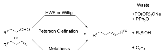
Scheme 1. Common homologation methodologies for the preparation of unsaturated compounds.
