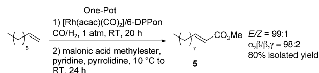
Scheme 6. An example of a one-pot RTAP hydroformylation/Knoevenagel reaction to \alpha,\beta -unsaturated carboxylic ester 5 .
