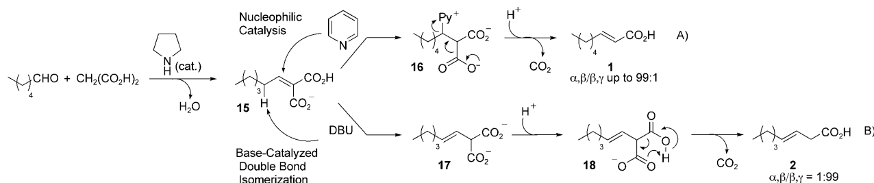
Scheme 13. Proposed mechanism, which is dependent upon the base used.
