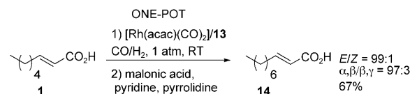
Scheme 12. One-pot C2 homologation of oct-2-enoic acid 1 .
