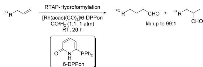
Scheme 2. RTAP hydroformylation–atom-economic C1 homologation.
