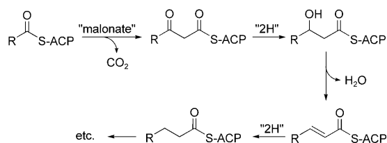
Scheme 11. Biosynthesis of fatty acids.
