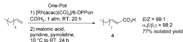
Scheme 5. An example of a one-pot RTAP hydroformylation/Knoevenagel reaction to \alpha,\beta -unsaturated carboxylic acid 4 .
